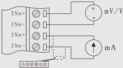
CK-8082R analog input wiring diagram
